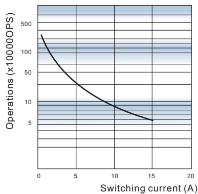
Electrical endurance curve
